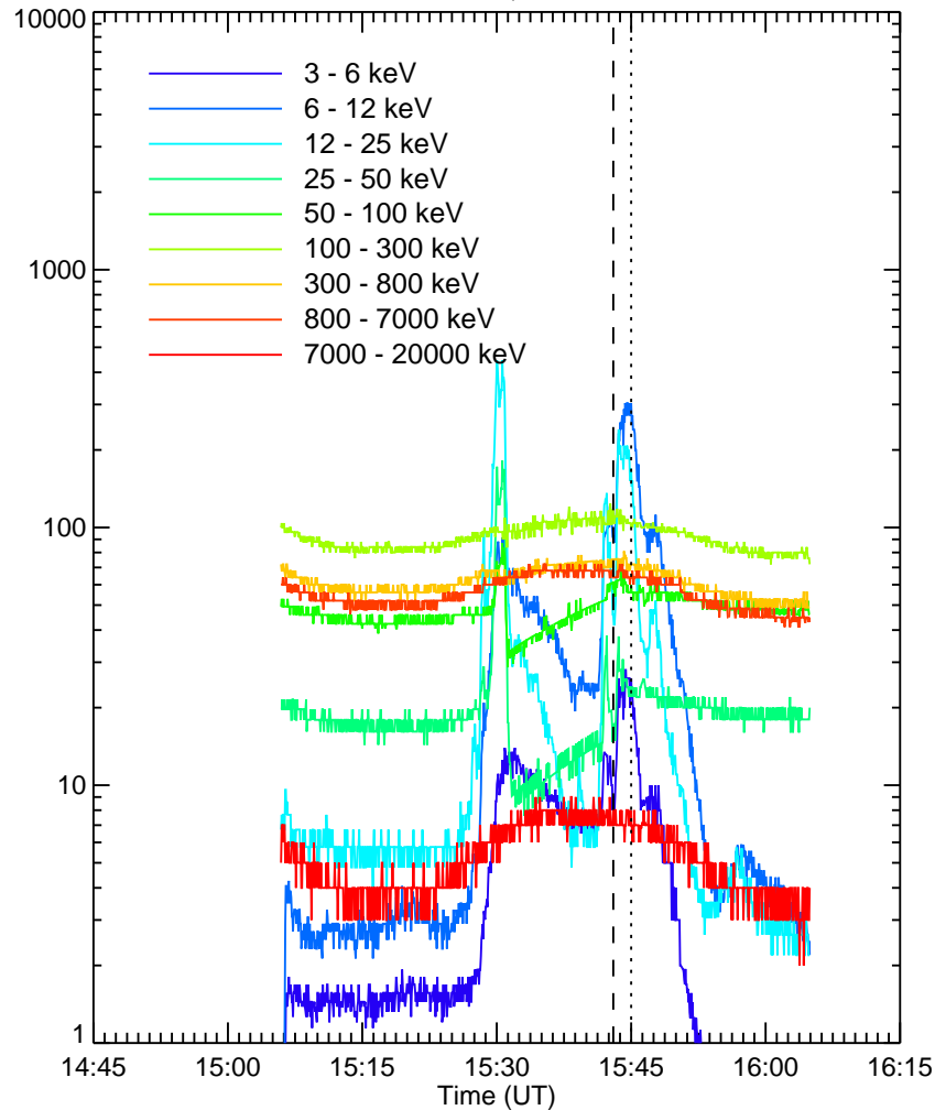
RHESHI Quicklook
