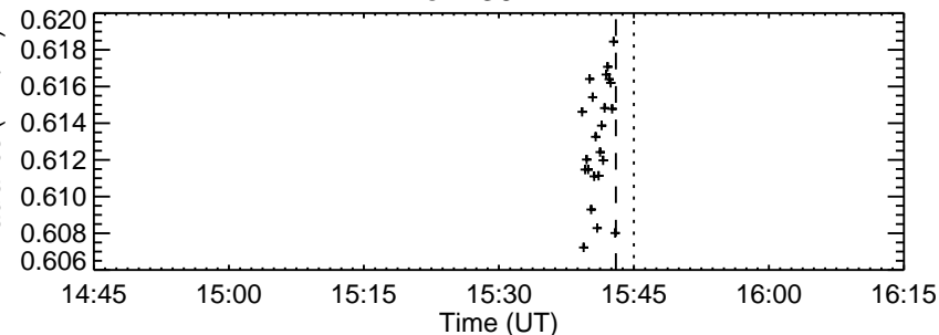
RHESHI Quicklook
