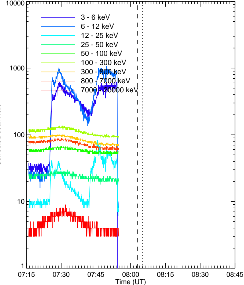
RHESSI Quicklook
