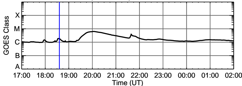
16-Jul-2012 (DOY 198) C1.8 @ 18:36:00 UT
