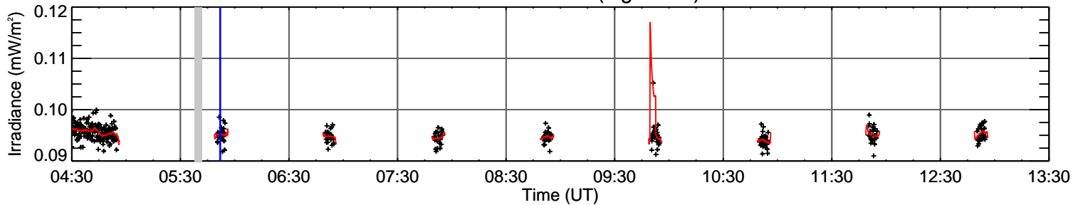
EVE H I 102.6 nm (log T=3.8)
