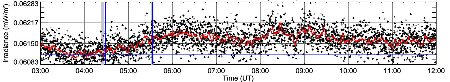
EVE Fe XI 18.0 nm (log T=6.1)
