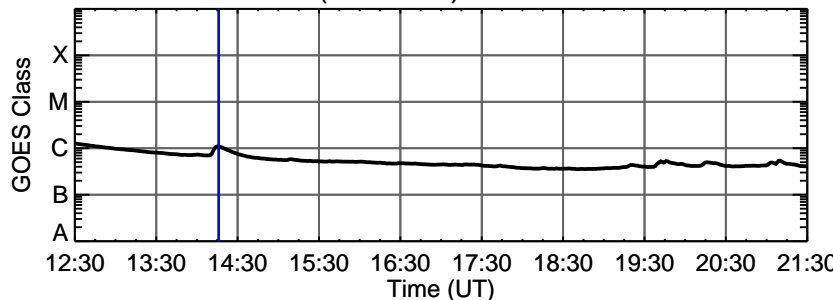
12-Mar-2013 (DOY 071) C1.0 @ 14:16:00 UT
