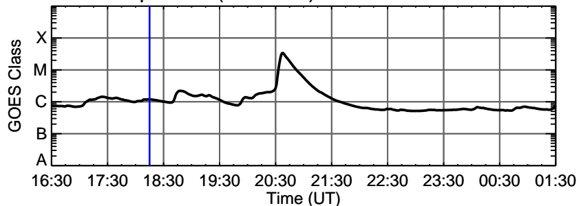
12-Apr-2013 (DOY 102) C1.1 @ 18:15:00 UT
