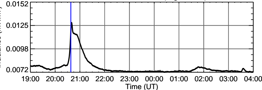
EVE Fe XVI 33.5 nm (log T=6.4)
