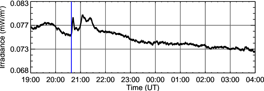
EVE Fe XV 28.4 nm (log T=6.3)
