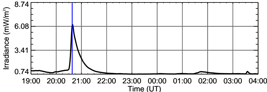
EVE Fe XX 13.3 nm (log T=7.0)
