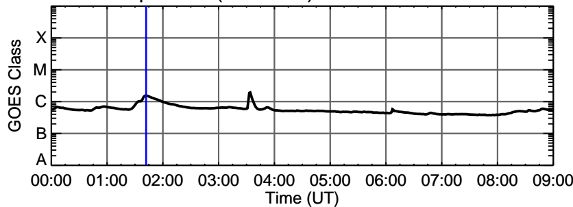
13-Apr-2013 (DOY 103) C1.5 @ 01:42:00 UT
