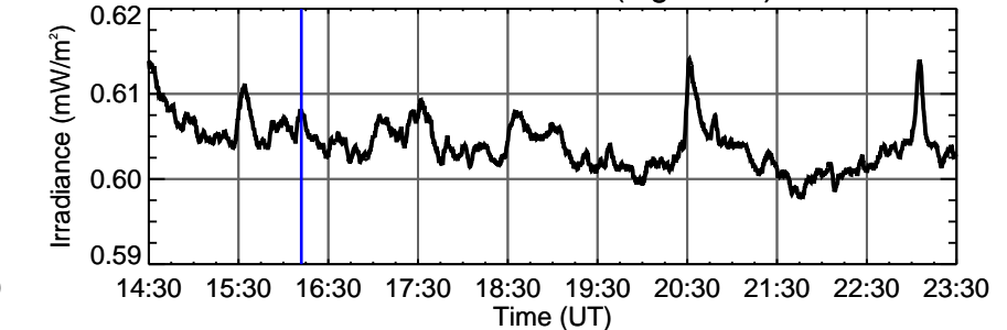
ESP 30.4 nm
