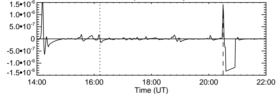
He II 30.4 nm
