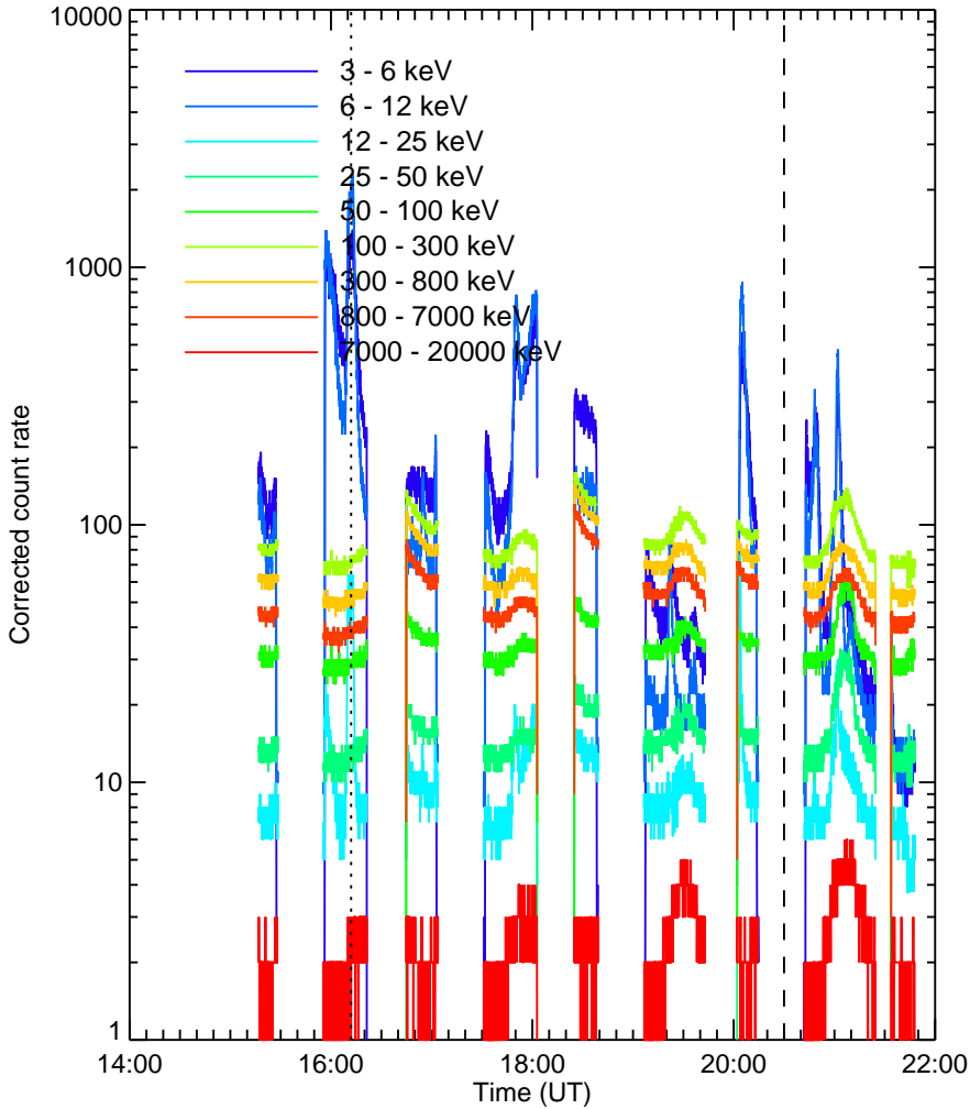
RHESSEI Quicklook
