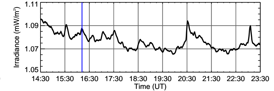
ESP 30.4 nm
