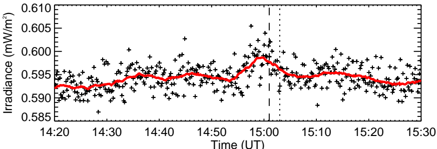
RHESSEI Quicklook
