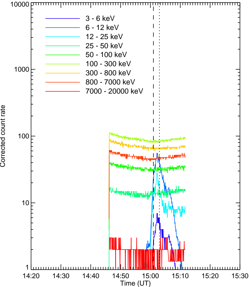
RHESSEI Quicklook
