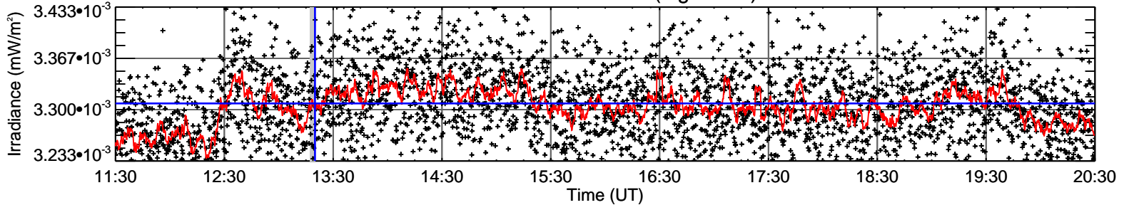
EVE Fe VIII 13.1 nm (log T=5.6)
