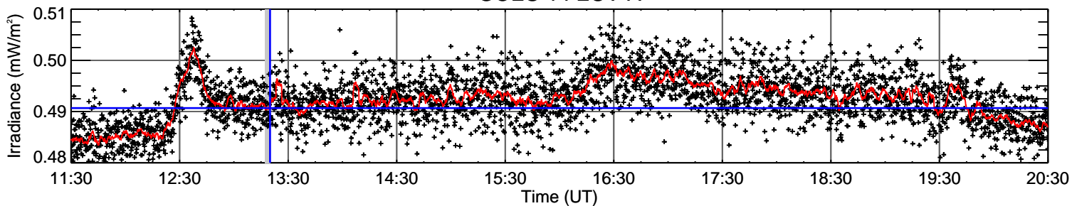
GOES-14 EUV-B
