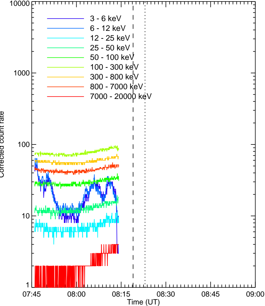
RHESSI Quicklook
