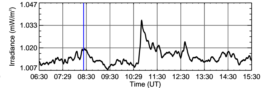
ESP 30.4 nm
