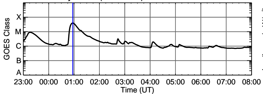
10-May-2013 (DOY 130) M3.9 @ 00:57:00 UT
