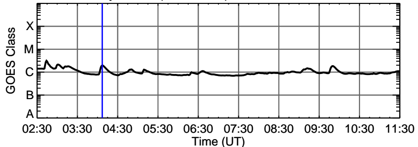
10-May-2013 (DOY 130) C1.9 @ 04:07:00 UT
