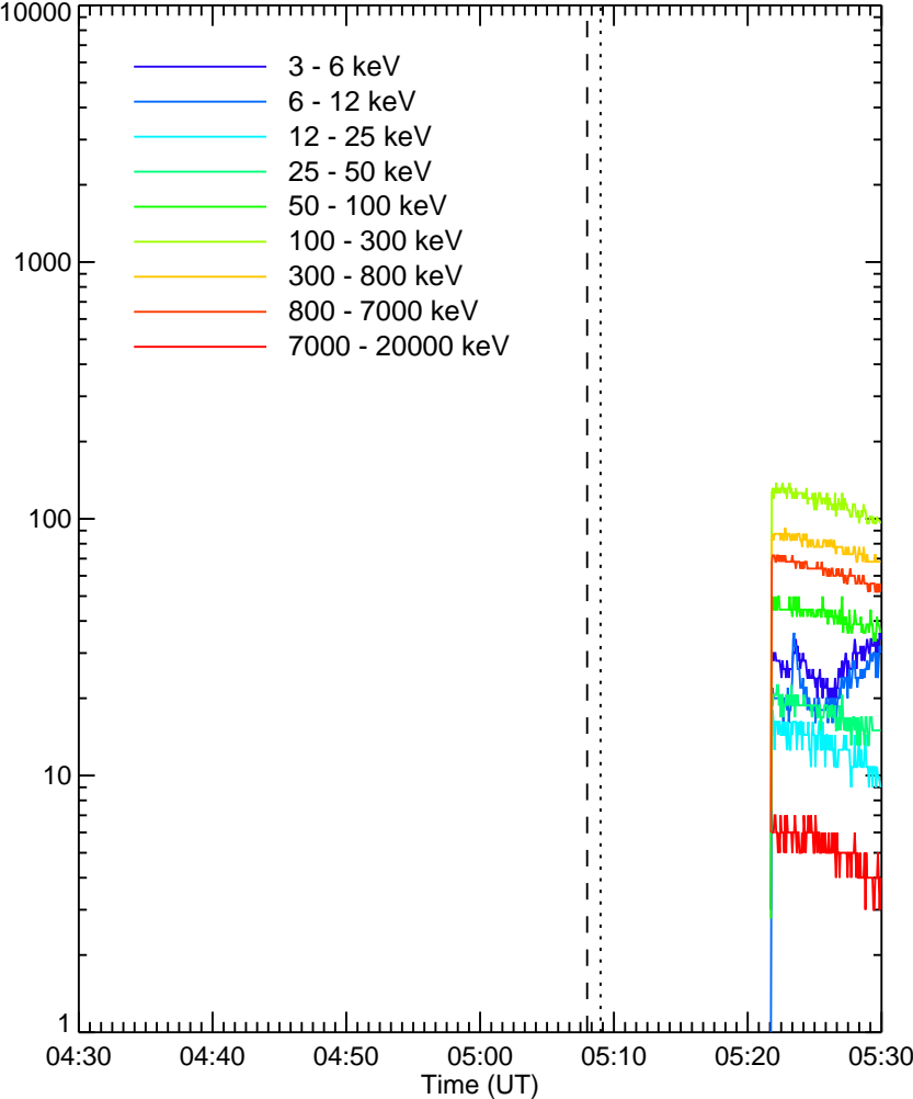
RHESSI Quicklook
