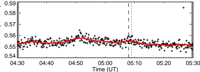
RHESSI Quicklook
