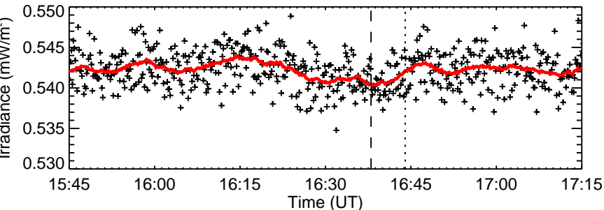
RHESSE Quicklook
