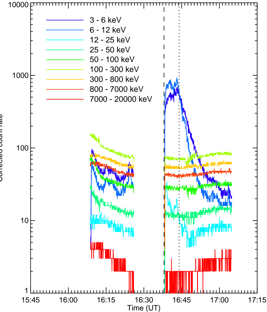
RHESSE Quicklook
