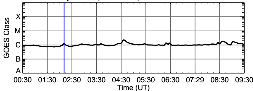
12-May-2013 (DOY 132) C1.2 @ 02:11:00 UT
