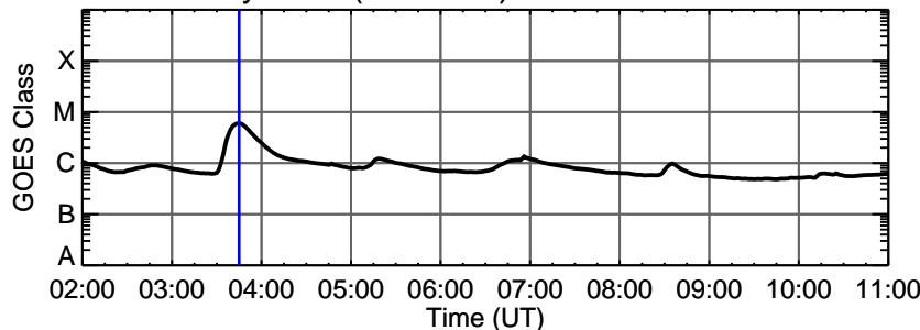
18-May-2013 (DOY 138) C6.0 @ 03:45:00 UT
