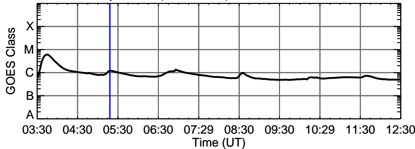
18-May-2013 (DOY 138) C1.2 @ 05:18:00 UT
