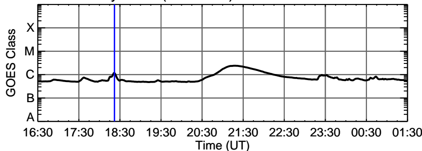
18-May-2013 (DOY 138) C1.1 @ 18:22:00 UT
