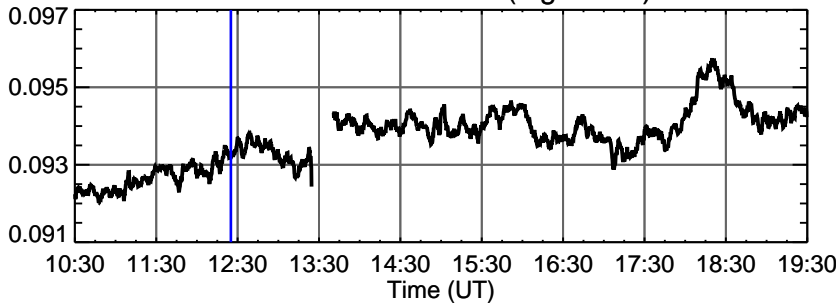
EVE Fe XV 28.4 nm (log T=6.3)
