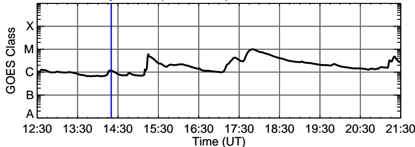
19-May-2013 (DOY 139) C1.1 @ 14:20:00 UT
