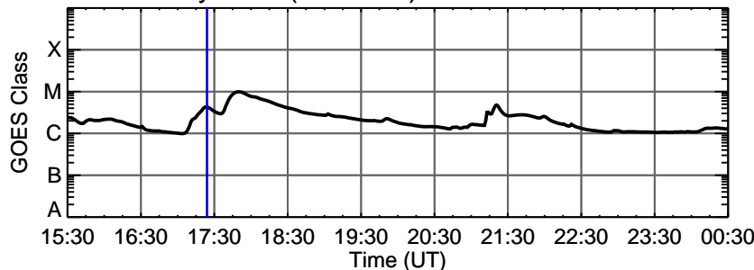
19-May-2013 (DOY 139) C4.2 @ 17:24:00 UT
