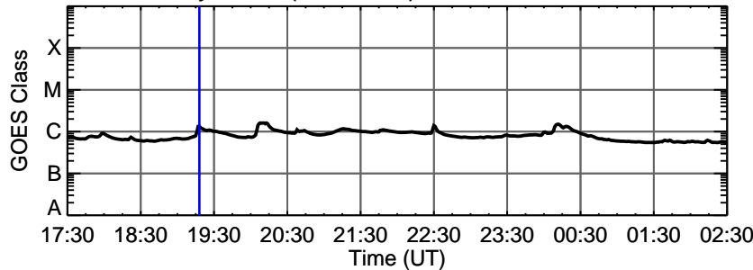
20-May-2013 (DOY 140) C1.3 @ 19:18:00 UT
