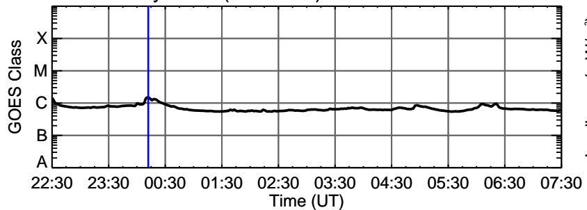
21-May-2013 (DOY 141) C1.5 @ 00:12:00 UT
