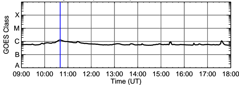
21-May-2013 (DOY 141) C1.2 @ 10:40:00 UT
