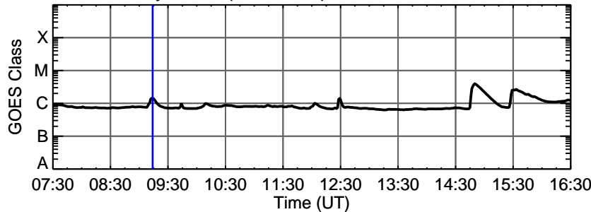
23-May-2013 (DOY 143) C1.4 @ 09:14:00 UT
