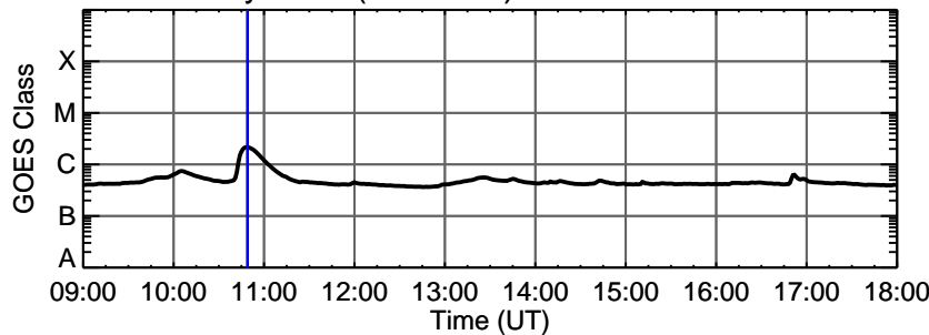
25-May-2013 (DOY 145) C2.1 @ 10:49:00 UT
