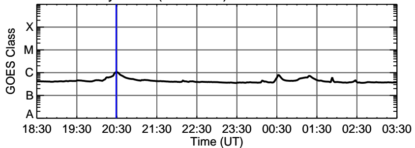
25-May-2013 (DOY 145) C1.6 @ 20:29:00 UT
