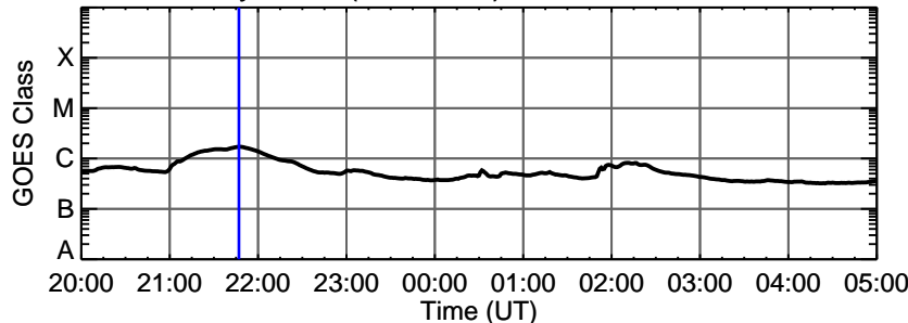
26-May-2013 (DOY 146) C1.7 @ 21:47:00 UT
