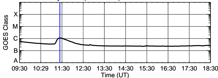
31-May-2013 (DOY 151) C1.1 @ 11:24:00 UT
