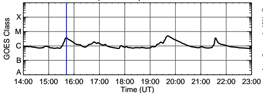
05-Jul-2013 (DOY 186) C3.6 @ 15:42:00 UT
