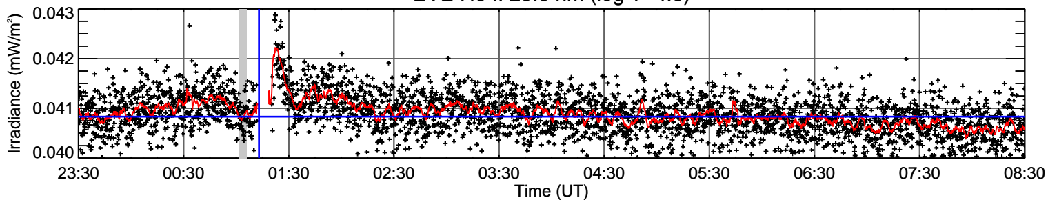
EVE He II 30.4 nm (log T=4.7)
