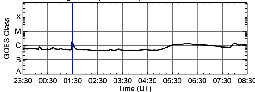
20-Aug-2013 (DOY 232) C1.8 @ 01:29:00 UT
