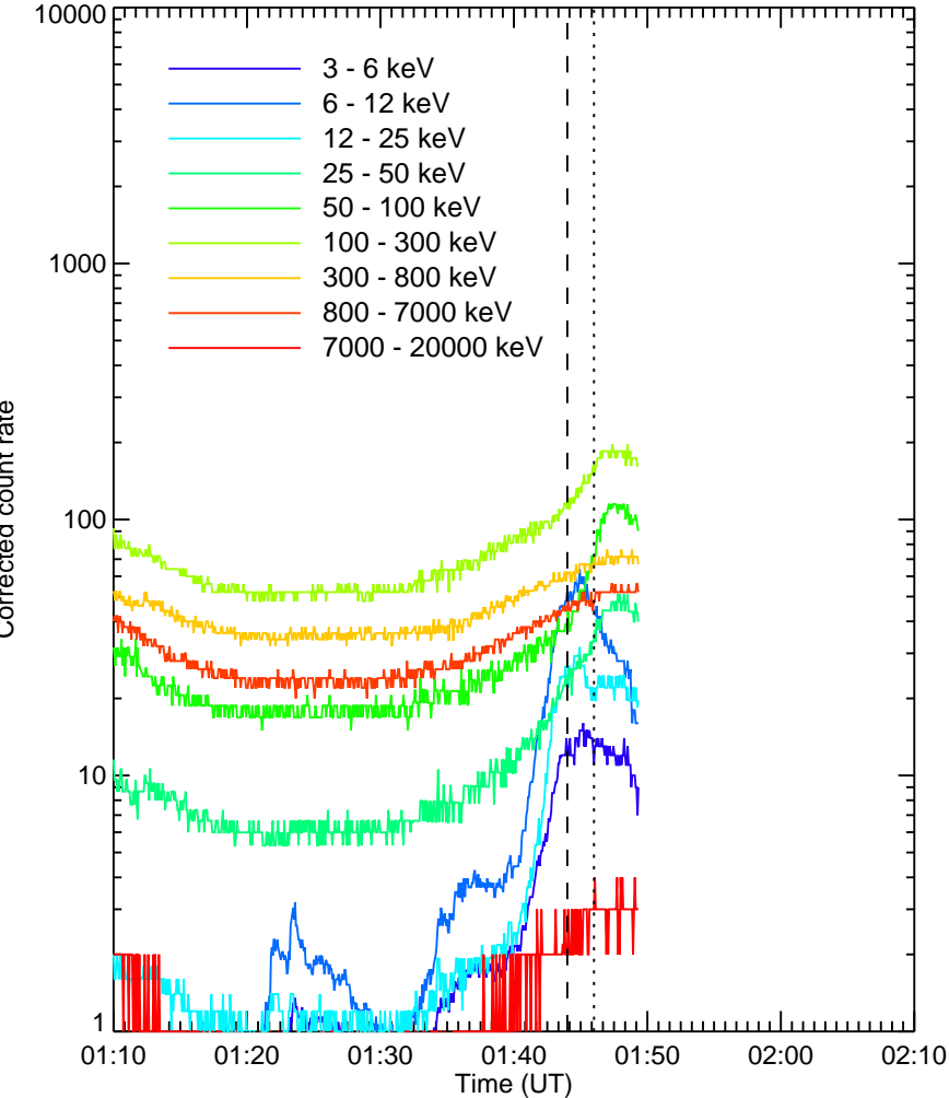
RHESSEI Quicklook
