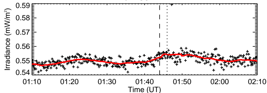
RHESSEI Quicklook
