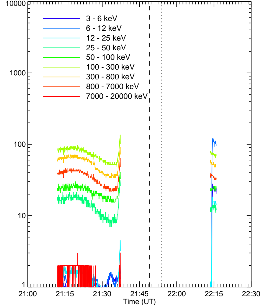
RHESSI Quicklook
