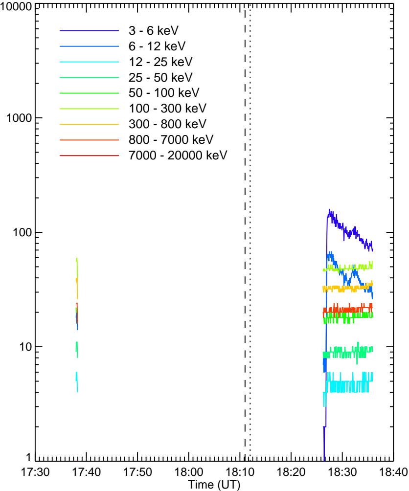
RHESSI Quicklook
