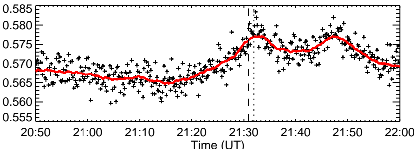
RHESSEI Quicklook
