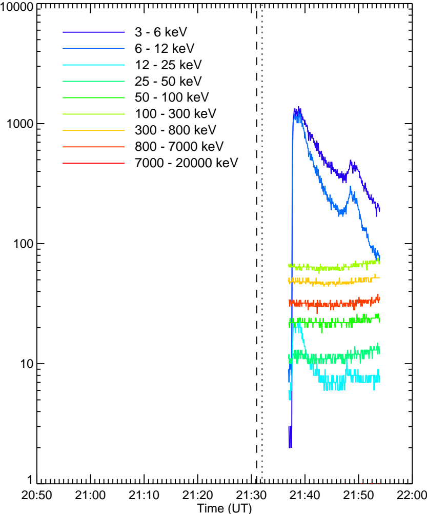
RHESSEI Quicklook
