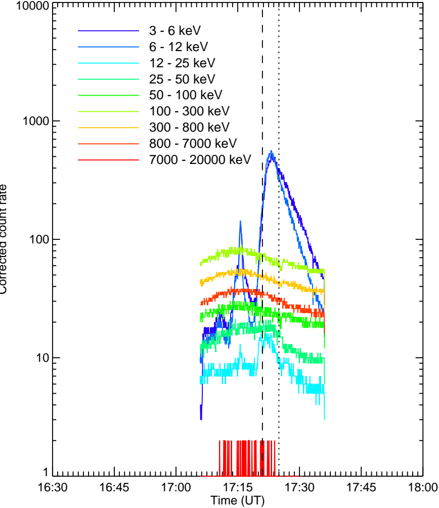
RHESHI Quicklook
