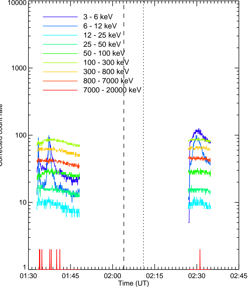
RHESSEI Quicklook
