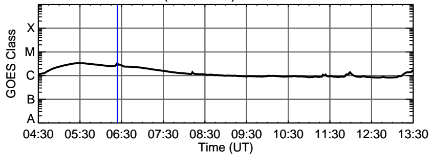
12-Nov-2013 (DOY 316) C3.2 @ 06:24:00 UT
