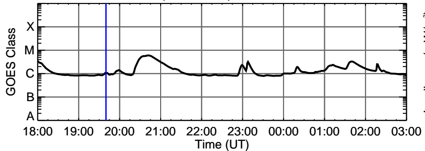
13-Nov-2013 (DOY 317) C1.0 @ 19:40:00 UT
