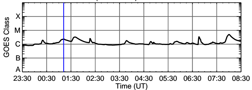
14-Nov-2013 (DOY 318) C2.3 @ 01:12:00 UT
