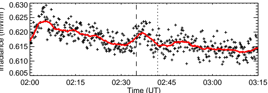
RHESSEI Quicklook
