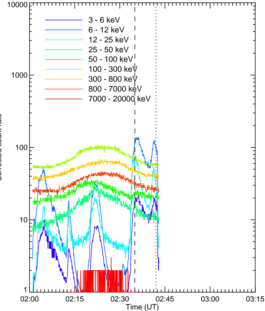
RHESSEI Quicklook
