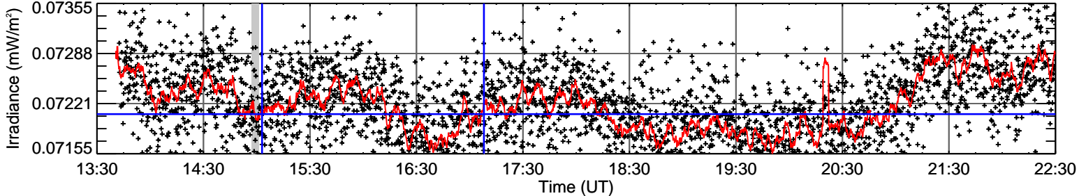
EVE Ne VII 46.5 nm (log T=5.7)
