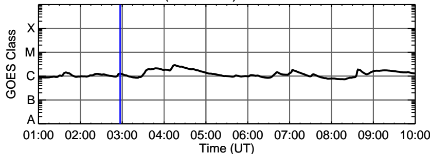
18-Nov-2013 (DOY 322) C1.2 @ 02:57:00 UT
