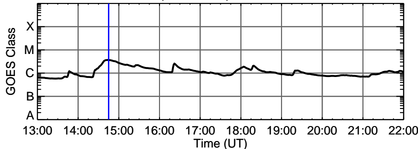
22-Nov-2013 (DOY 326) C3.6 @ 14:45:00 UT
