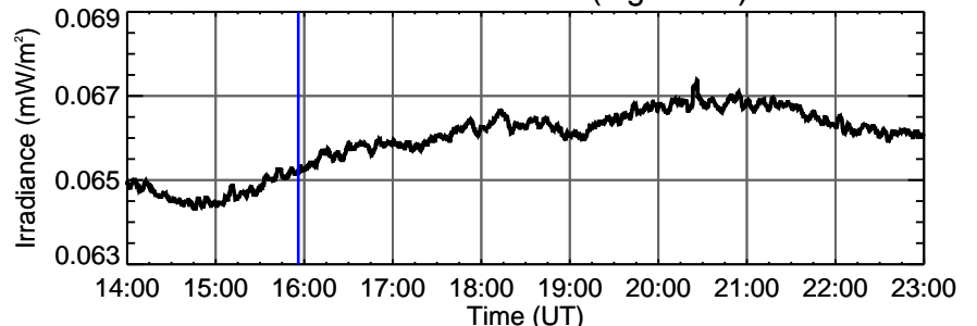
EVE He II 30.4 nm (log T=4.7)
