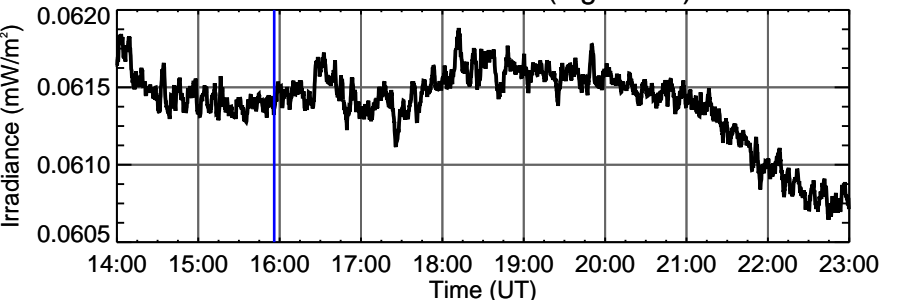
EVE Fe X 17.7 nm (log T=6.0)
