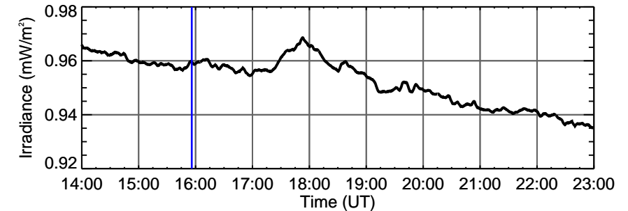
ESP 30.4 nm
