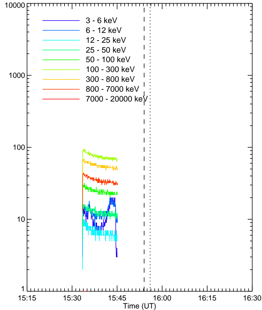
RHESSI Quicklook
