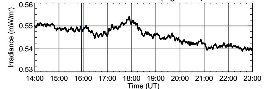
ESP 30.4 nm
