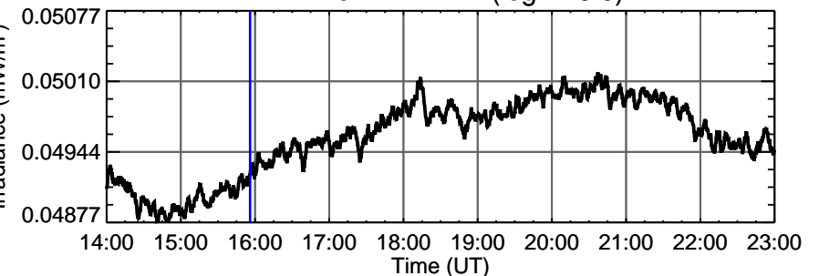
EVE Fe IX 17.1 nm (log T=5.8)
