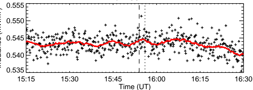
RHESSI Quicklook
