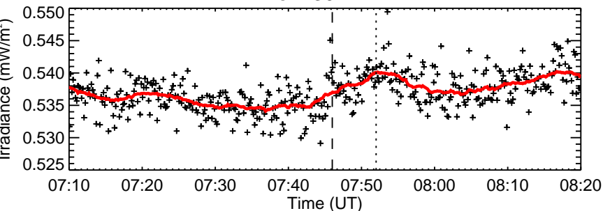
RHESHI Quicklook
